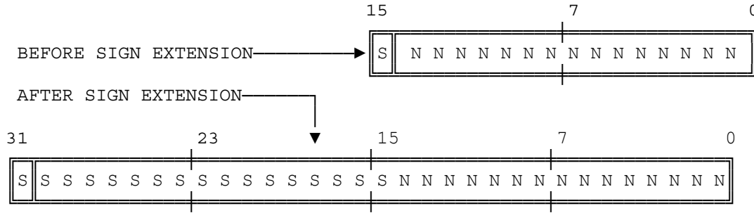
Figure 3-5. Sign Extension
