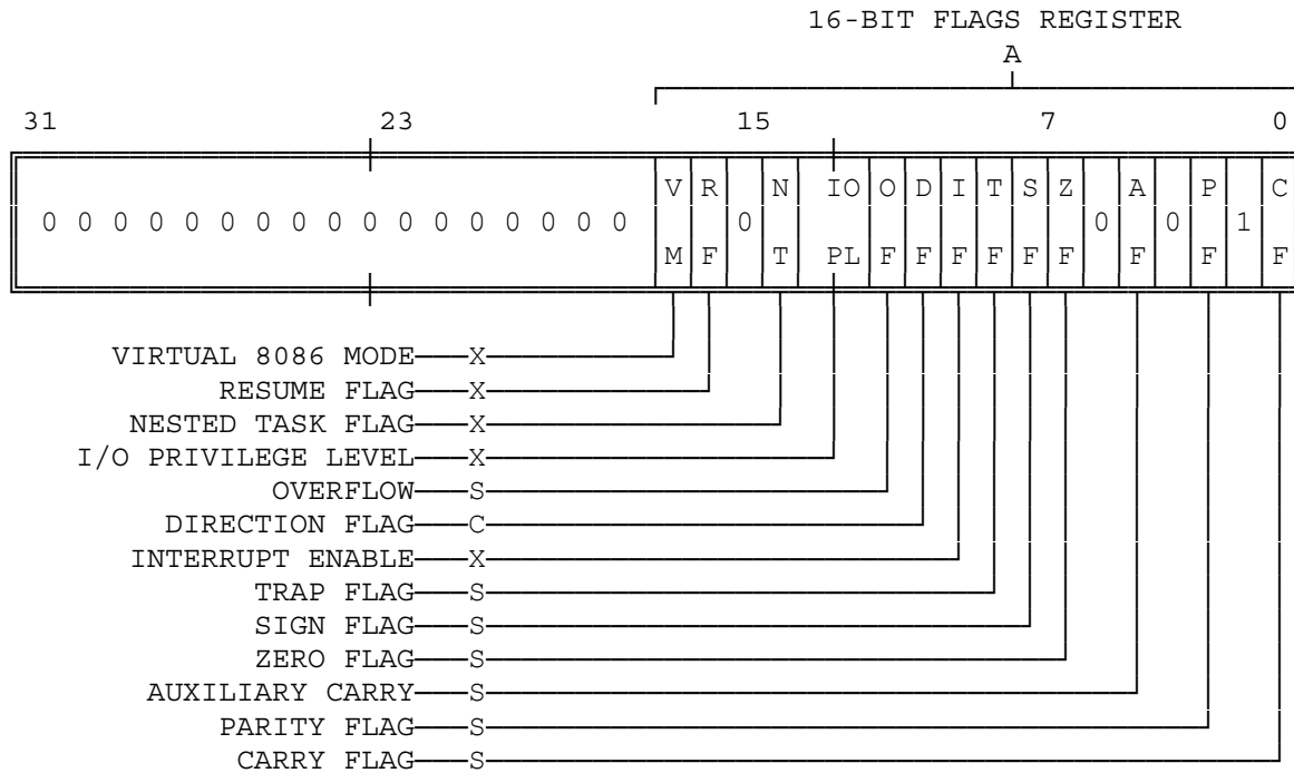
Figure 2-8. EFLAGS Register
