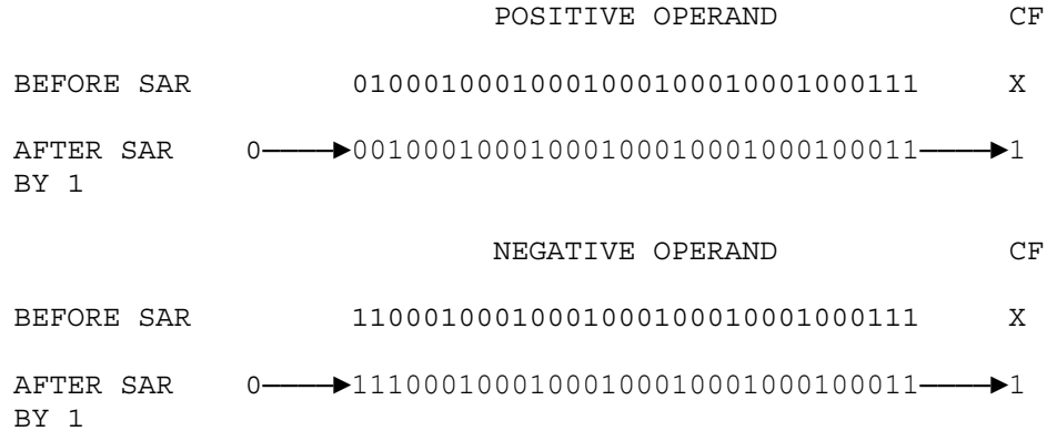
Figure 3-8. SAR
