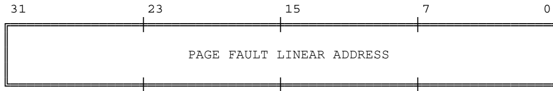
Figure 9-9. CR2 Format
