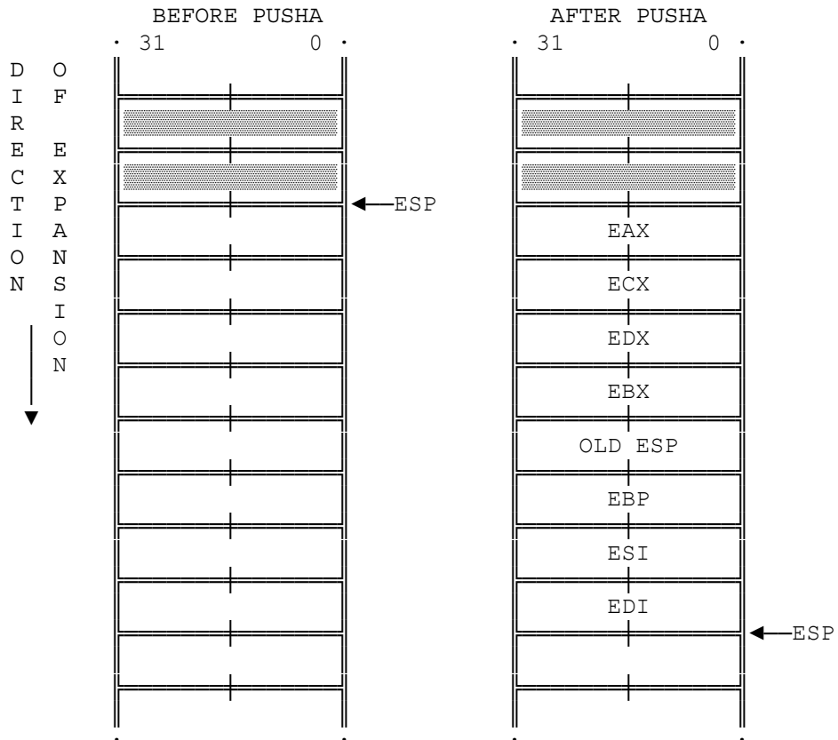
Figure 3-2. PUSHA
