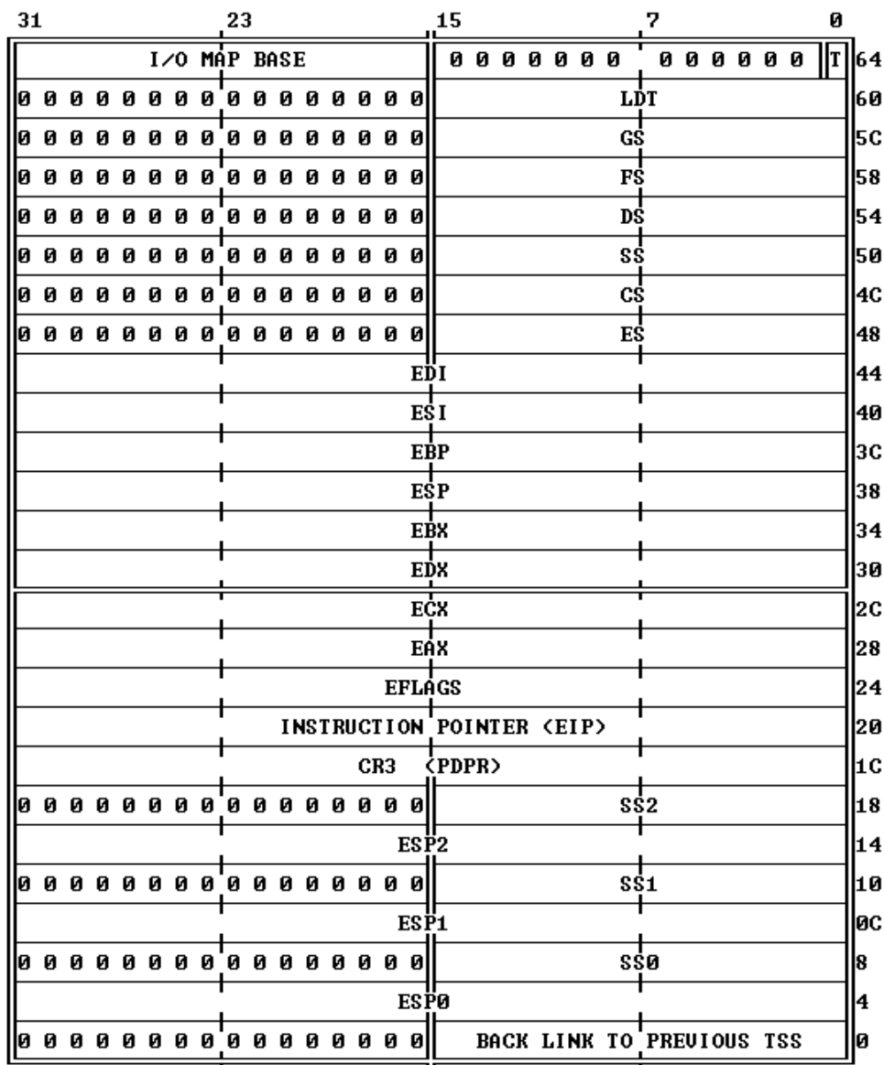
Figure 7-1. 80386 32-Bit Task State Segment
