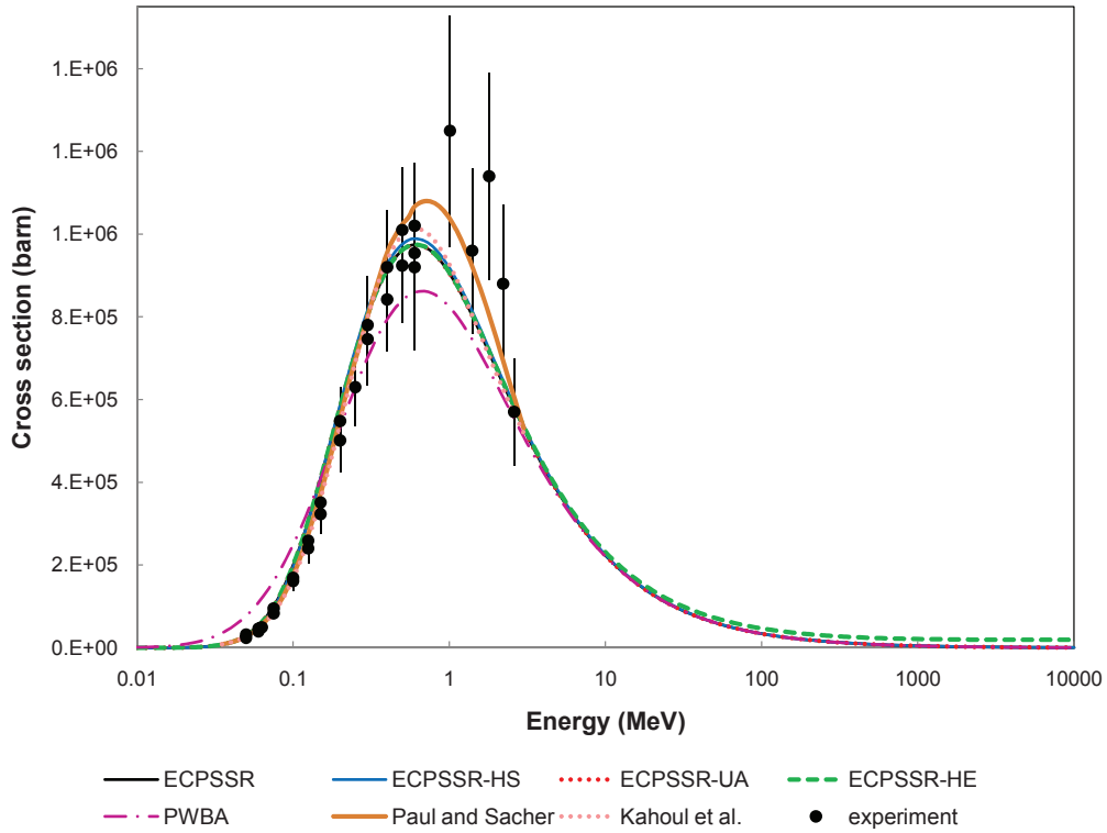
Figure 20.2: Cross section for the ionisation of carbon K shell by proton impact according to the various implemented modeling options, and comparison with experimental data [23]: ECPSSR model, ECPSSR model with “united atom” (UA) approximation, Hartree-Slater (HS) corrections and specialized for high energies (HE); plane wave Born approximation (PWBA); empirical models by Paul and Sacher and Kahoul et al. The curves reproducing some of the model implementations can be hardly distinguished in the plot due to their similarity.
