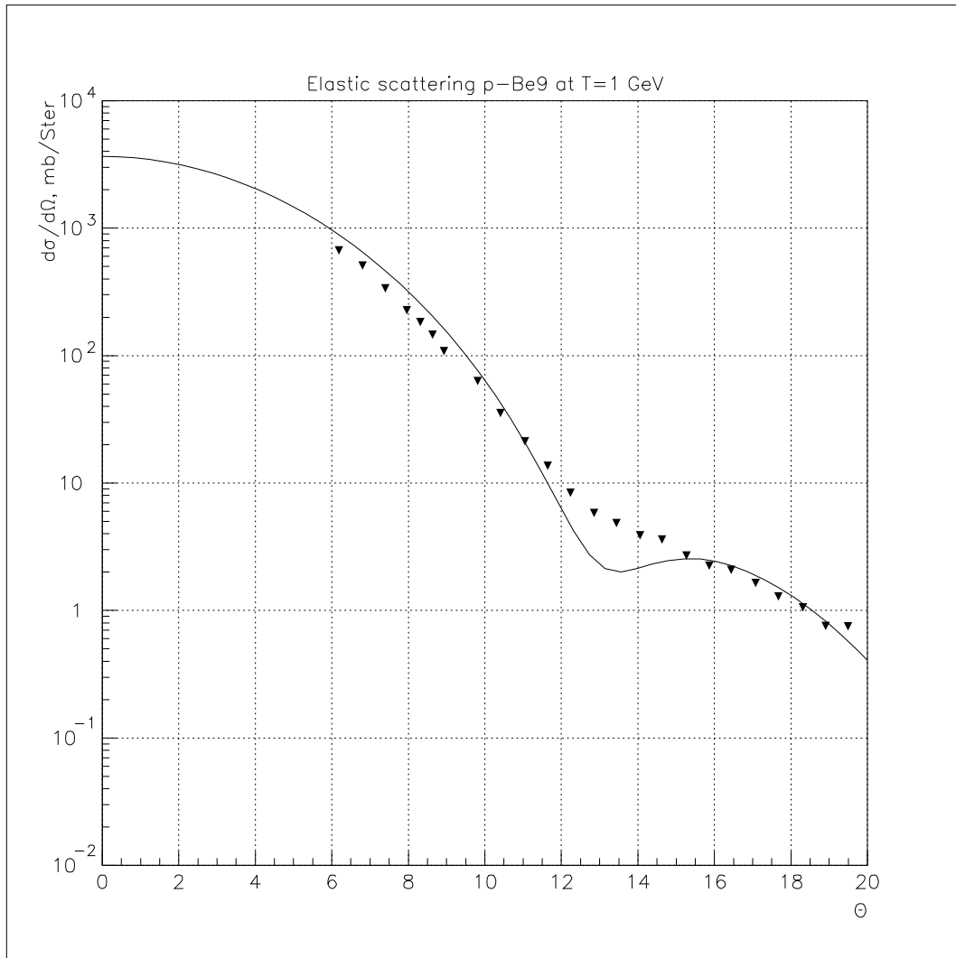
Figure 24.1: Elastic proton scattering on {}^9\text{Be} at 1 GeV
