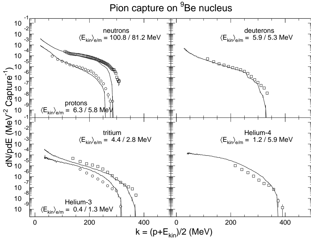
Figure 28.8: Comparison of the CHIPS model results with experimental data on proton, neutron, and nuclear fragment production in the capture of negative pions on {}^9\text{Be} . Proton [47] and neutron [49] experimental spectra are shown in the upper left panel by open circles and open squares, respectively. The model calculations are shown by the two corresponding solid lines. The same arrangement is used to present {}^3\text{He} [47] and tritium [47] spectra in the lower left panel. Deuterium [47] and {}^4\text{He} [47] spectra are shown in the right panels of the figure by open squares and lines (CHIPS model). The average kinetic energy carried away by each nuclear fragment is shown in the panels by the two numbers: first is the average calculated using the experimental data shown; second is the model result.
