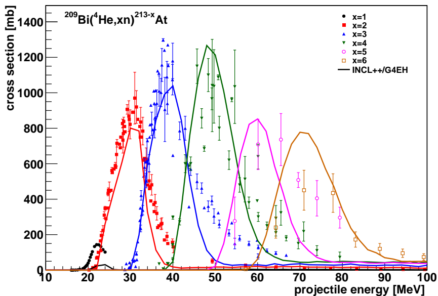
Figure 38.2: Excitation functions for (\alpha, xn) cross sections on ^{209}\text{Bi} . The predictions of INCL++-G4ExcitationHandler are represented by the solid line and are compared to experimental data [6, 7, 8, 9, 10, 11, 12, 13, 14].
