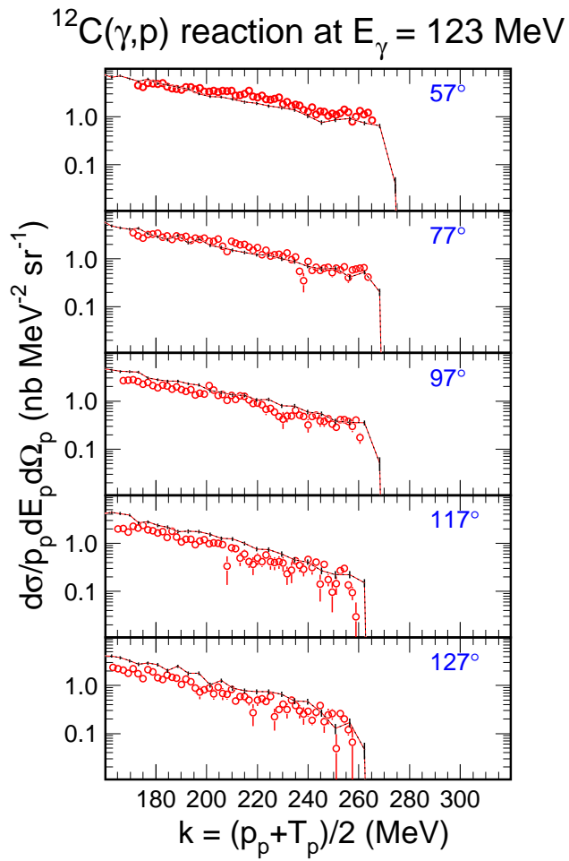
Figure 28.17: Comparison of the CHIPS model results (lines) with the experimental data [55] on proton spectra at 57^\circ , 77^\circ , 97^\circ , 117^\circ , and 127^\circ in the photonuclear reactions on ^{12}\text{C} at 123 MeV (open circles). The value of the total photonuclear cross section was set to 1.8 mb.
