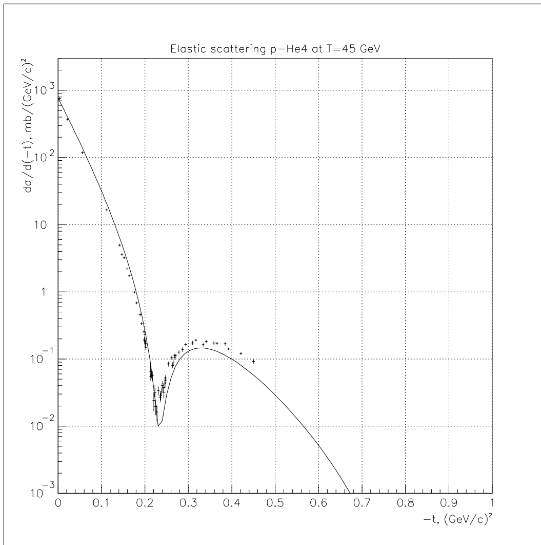
Figure 24.11: Elastic proton scattering on ^4\text{He} at 45 GeV
