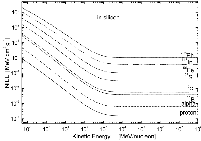
Figure 6.3: Non-ionizing stopping power from Ref. [1] - in \text{MeV cm}^2 \text{g}^{-1} - calculated using Eq. (6.82) in silicon is shown as a function of the kinetic energy per nucleon - from 50 keV/nucleon up 100 TeV/nucleon - for protons, \alpha -particles and ^{11}\text{B} -, ^{12}\text{C} -, ^{28}\text{Si} -, ^{56}\text{Fe} -, ^{115}\text{In} -, ^{208}\text{Pb} -nuclei. The threshold energy for displacement is 21 eV in silicon.
