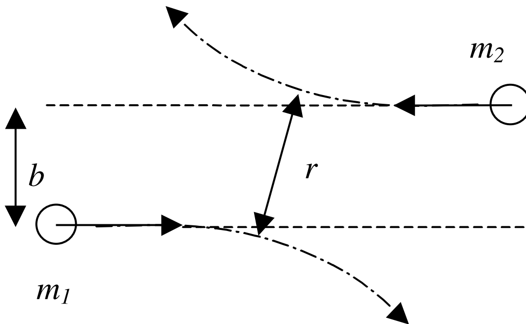
Figure 31.2: Illustration clarifying impact parameter in the far-field ( b ) and actual impact parameter ( r ).
