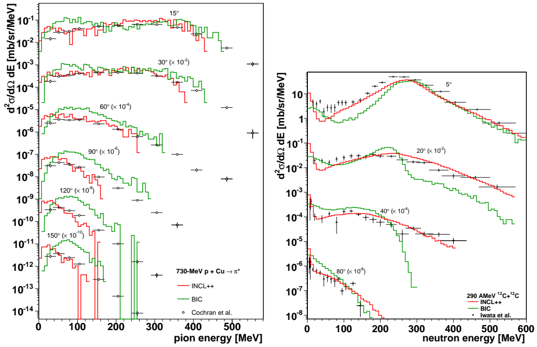
Figure 38.1: Left: double-differential cross sections for the production of charged pions in 730-MeV p+\text{Cu} . Right: double-differential cross sections for the production of neutrons in 290-AMeV ^{12}\text{C}+^{12}\text{C} . Predictions of the INCL++ and Binary-Cascade models are compared with experimental data from Refs. [4] and [5].
