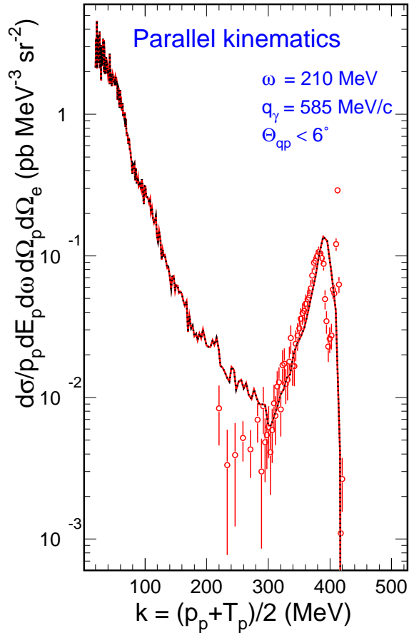
Figure 28.19: Comparison of the CHIPS model results (line) with the experimental data [56] (open circles) on the proton spectrum measured in parallel kinematics in the ^{12}\text{C}(e, e'p) reaction at an energy transfer equal to 210 MeV and momentum transfer equal to 585 MeV/c. Statistical errors in the CHIPS result are not shown but can be judged by the point-to-point variations in the line. The relative normalization is arbitrary.
