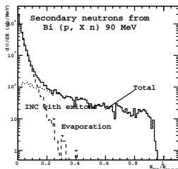
Figure 29.1: Secondary neutrons generated by Bertini INC with excitons and evaporation model.
