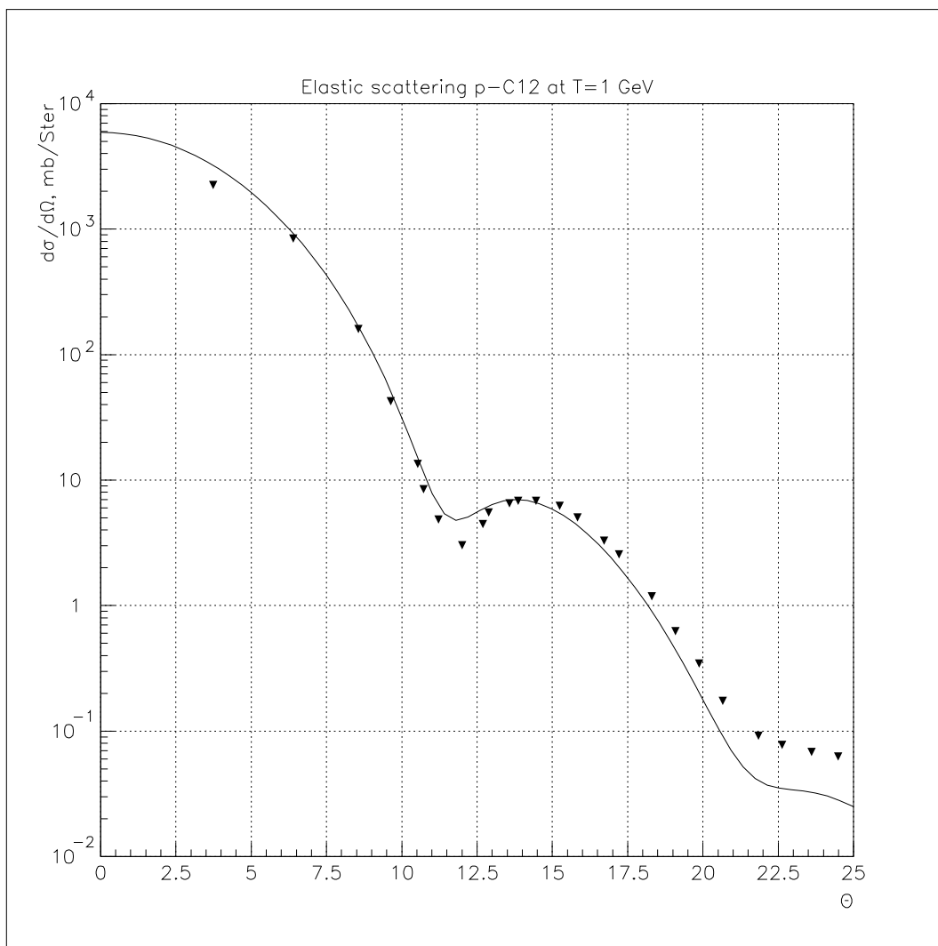
Figure 24.3: Elastic proton scattering on ^{12}\text{C} at 1 GeV
