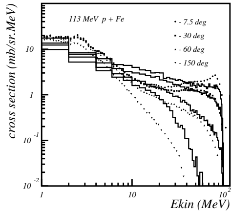
Figure 30.5: Double differential cross-section for neutrons produced in proton scattering off Iron. Proton incident energy was 113 MeV. The points are data, the histogram is Binary Cascade prediction.
