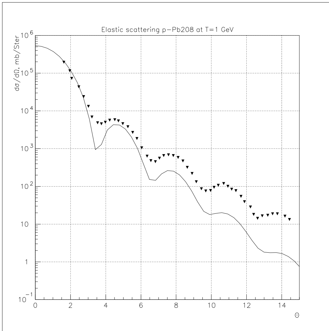
Figure 24.9: Elastic proton scattering on ^{208}\text{Pb} at 1 GeV
