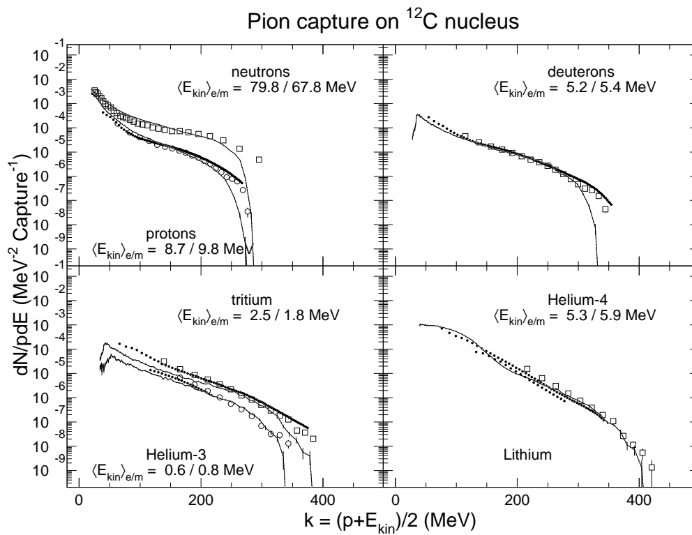
Figure 28.9: Same as in Figure 28.8, for pion capture on ^{12}\text{C} . The experimental neutron spectrum is taken from [50]. In addition, the detailed data on charged particle production, including the ^6\text{Li} spectrum, taken from Ref. [48], are superimposed on the plots as a series of dots.
