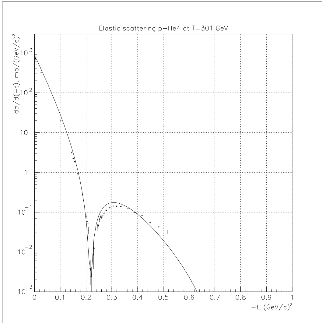
Figure 24.12: Elastic proton scattering on ^4\text{He} at 301 GeV
