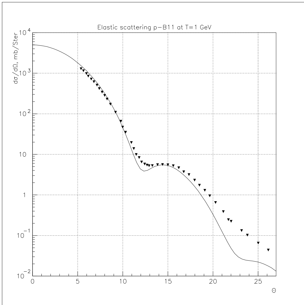
Figure 24.2: Elastic proton scattering on ^{11}\text{B} at 1 GeV
