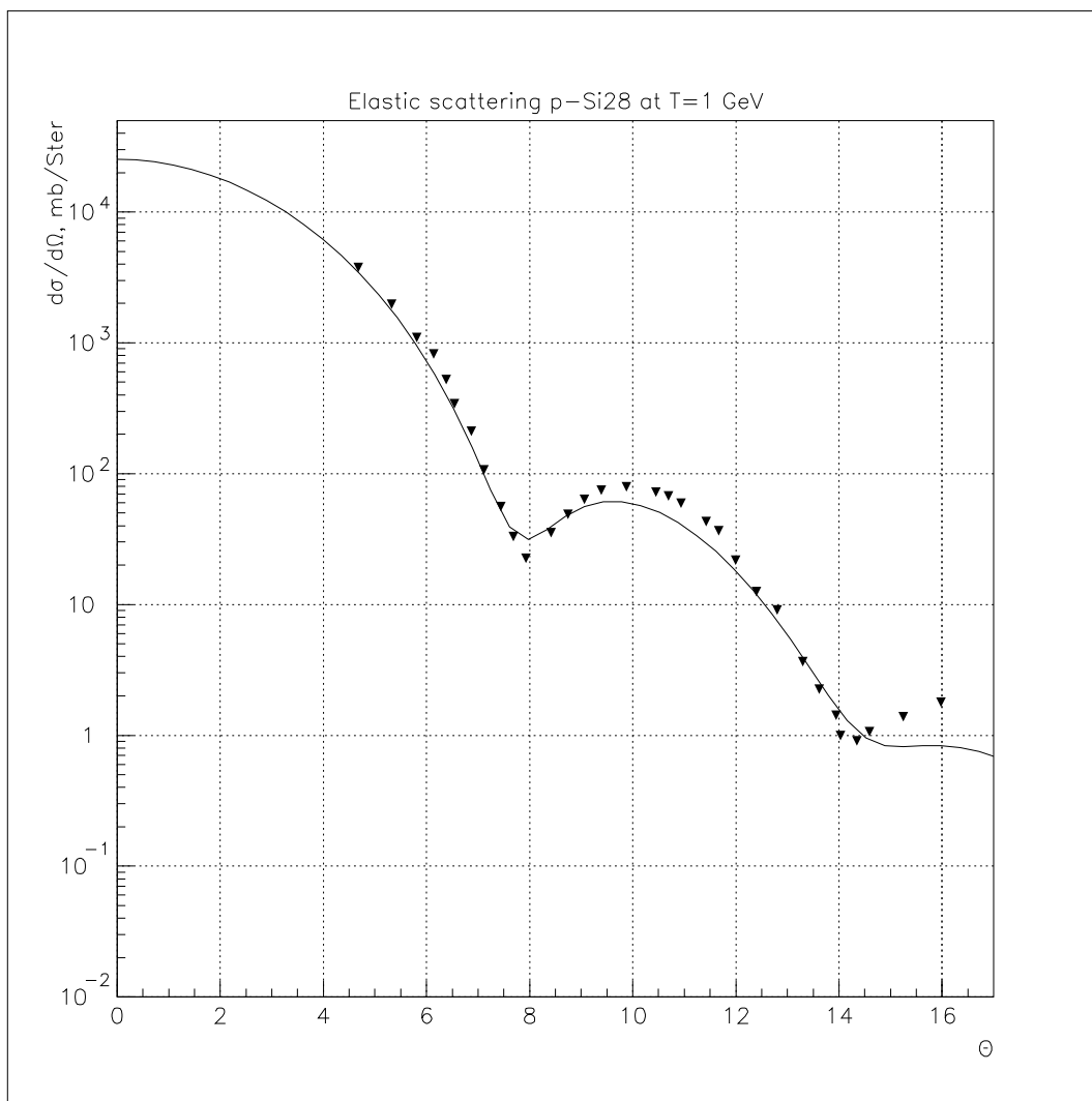
Figure 24.5: Elastic proton scattering on ^{28}\text{Si} at 1 GeV
