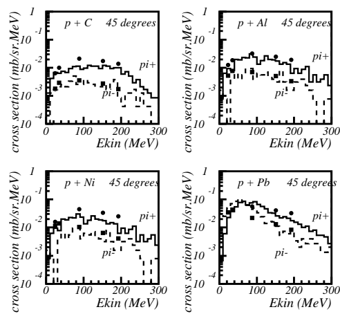
Figure 30.13: Double differential cross-section for pions produced at 45^\circ in proton scattering off various materials. Proton incident energy was 597 MeV in each case. The points are data, the histogram is Binary Cascade prediction.
