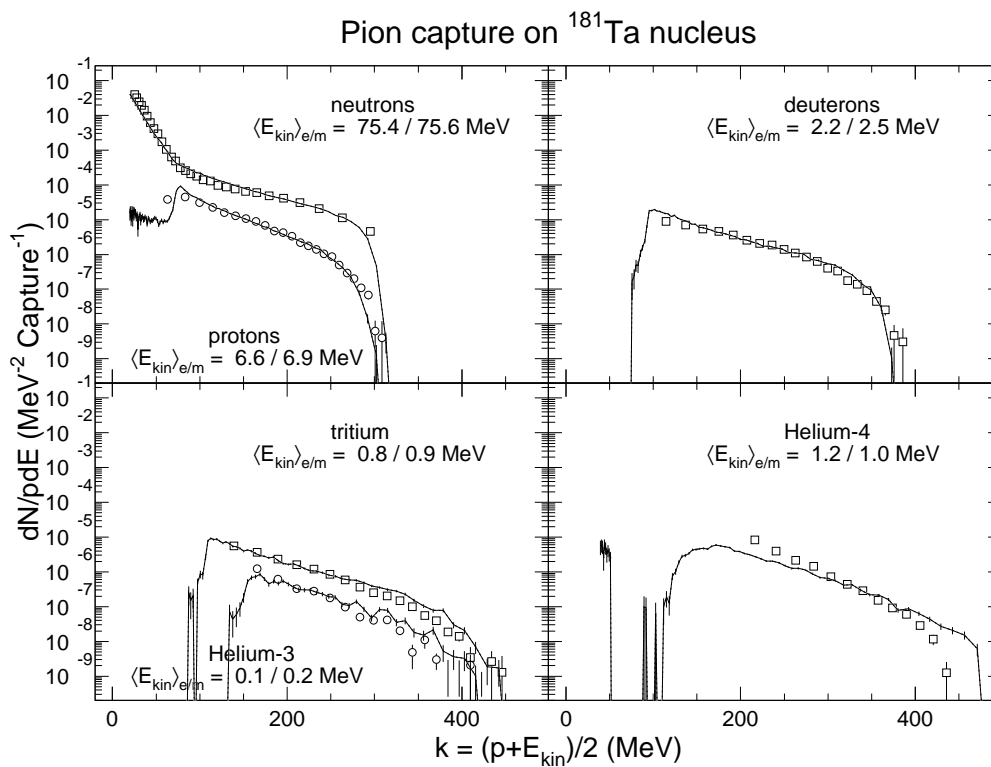
Figure 28.12: Same as in Figure 28.8, for pion capture on ^{181}\text{Ta} . The experimental neutron spectrum is taken from [50].
