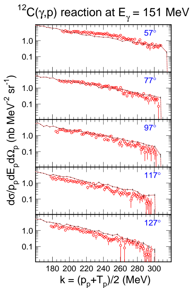
Figure 28.18: Same as in Fig. 28.17, for the photon energy 151 MeV.
