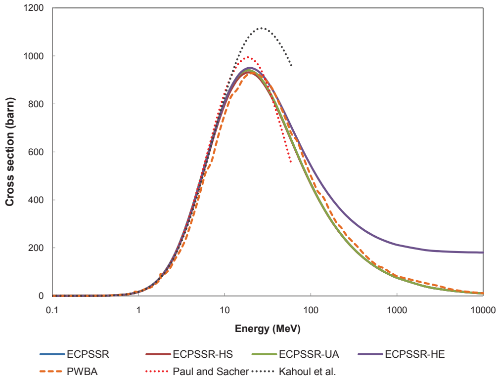
Figure 20.1: Cross section for the ionisation of copper K shell by proton impact according to the various implemented modeling options: ECPSSR model, ECPSSR model with “united atom” (UA) approximation, Hartree-Slater (HS) corrections and specialized for high energies (HE); plane wave Born approximation (PWBA); empirical models by Paul and Sacher and Kahoul et al. The curves reproducing some of the model implementations can be hardly distinguished in the plot due to their similarity.
