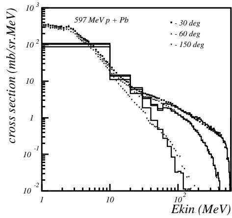
Figure 30.11: Double differential cross-section for neutrons produced in proton scattering off Lead. Proton incident energy was 597 MeV. The points are data, the histogram is Binary Cascade prediction.
