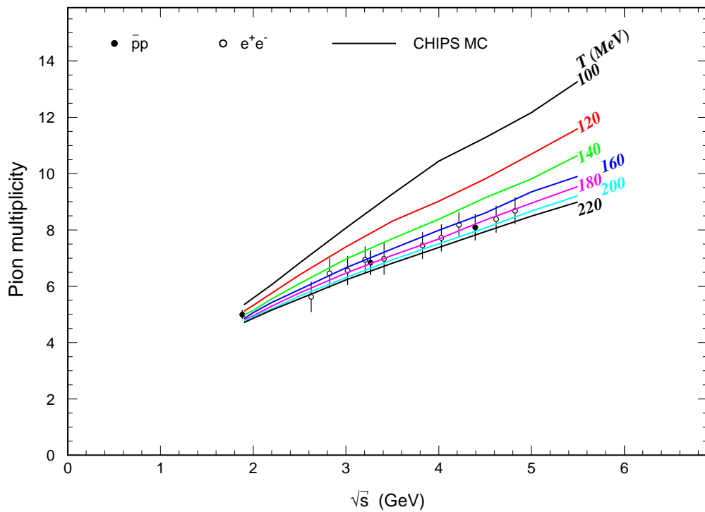
Figure 28.6: Average meson multiplicities in proton-antiproton and in electron-positron annihilation, as a function of the center-of-mass energy of the interacting hadronic system. The points are experimental data [21] and the lines are CHIPS Monte Carlo calculations at several values of the critical temperature parameter T .
