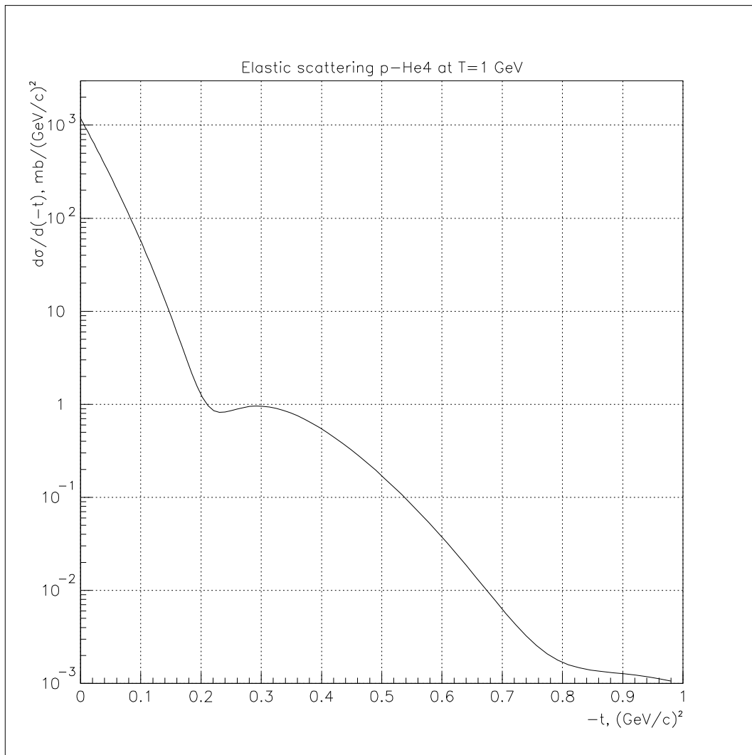
Figure 24.10: Elastic proton scattering on ^4\text{He} at 1 GeV
