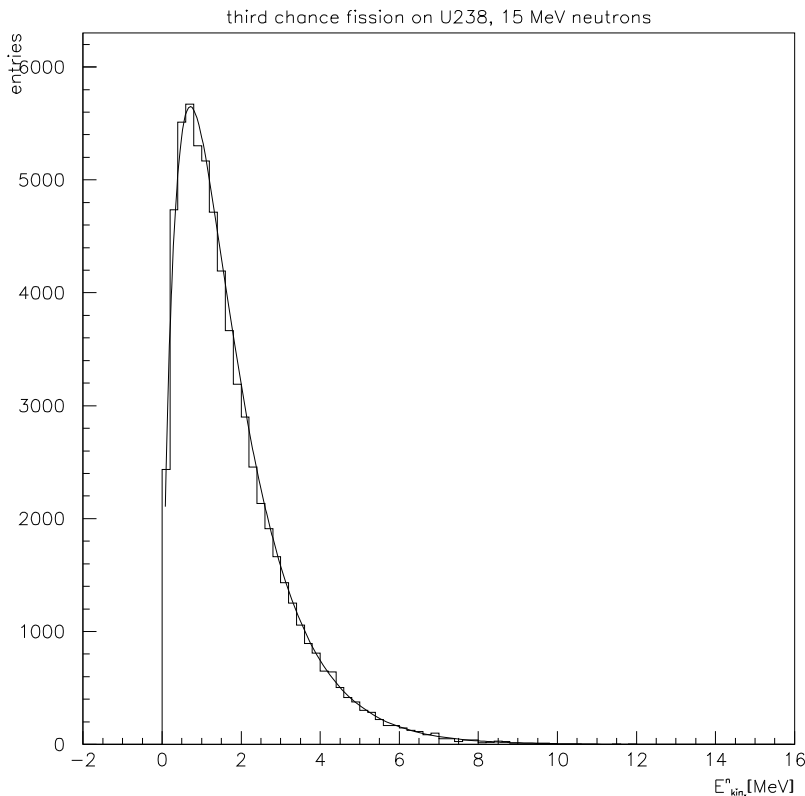
Figure 39.3: Comparison of data and Monte Carlo for fission neutron energy distributions for induced fission by 15 MeV neutrons on Uranium ( ^{238}\text{U} ). The curve represents evaluated data and the histogram is the Monte Carlo prediction.
