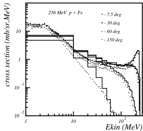
Figure 30.6: Double differential cross-section for neutrons produced in proton scattering off Iron. Proton incident energy was 256 MeV. The points are data, the histogram is Binary Cascade prediction.
