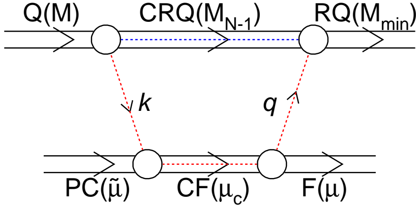
Figure 28.7: Diagram of the quark exchange mechanism.
