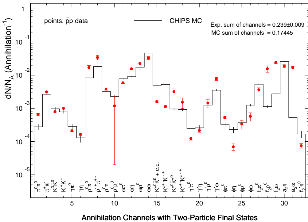
Figure 28.5: Branching probabilities for different channels with two-particle final states in proton-antiproton annihilation at rest. The points are experimental data [19] and the histogram is from the CHIPS Monte Carlo.
