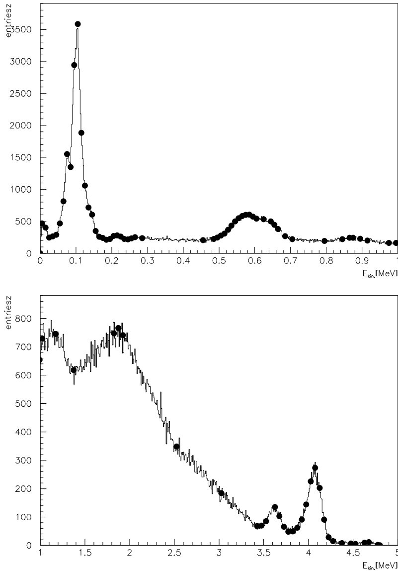
Figure 39.2: Comparison of data and Monte Carlo for photon energy distributions for radiative capture of 15 MeV neutrons on Uranium ( ^{238}\text{U} ). The points are evaluated data, the histogram is the Monte Carlo prediction.
