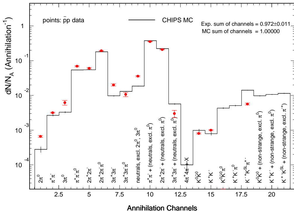
Figure 28.3: Branching probabilities for different channels in proton-antiproton annihilation at rest. The experimental data are from [19], and the histogram was produced by the CHIPS Monte Carlo.
