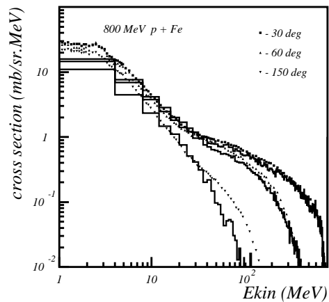
Figure 30.8: Double differential cross-section for neutrons produced in proton scattering off Iron. Proton incident energy was 800 MeV. The points are data, the histogram is Binary Cascade prediction.
